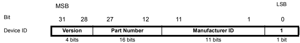
Figure 124. The Format of the Device Identification Register
