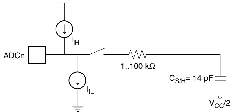
Figure 114. Analog Input Circuitry
