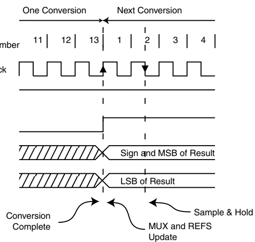
Figure 113. ADC Timing Diagram, Free Running Conversion
