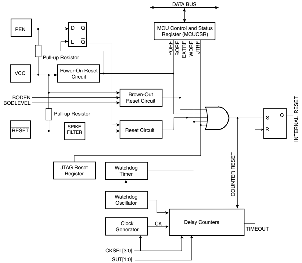
Figure 21. Reset Logic
