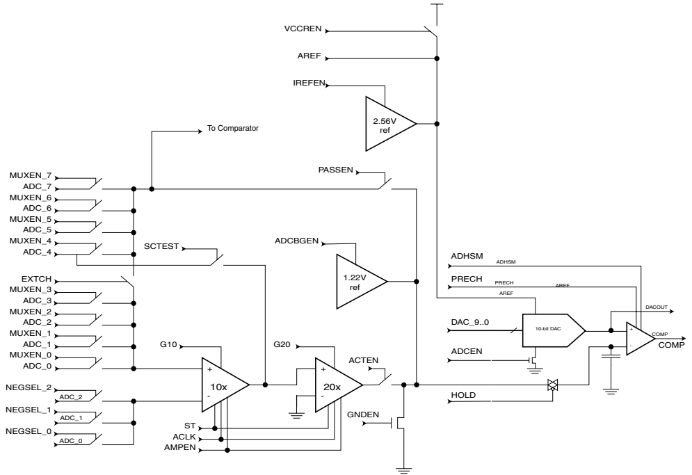
Figure 133. Analog to Digital Converter
