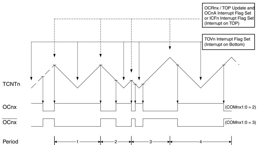
Figure 52. Phase Correct PWM Mode, Timing Diagram
