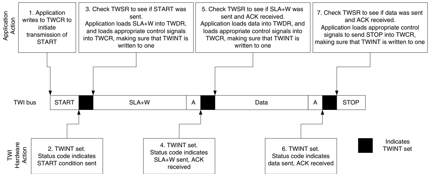
Figure 94. Interfacing the Application to the TWI in a Typical Transmission
