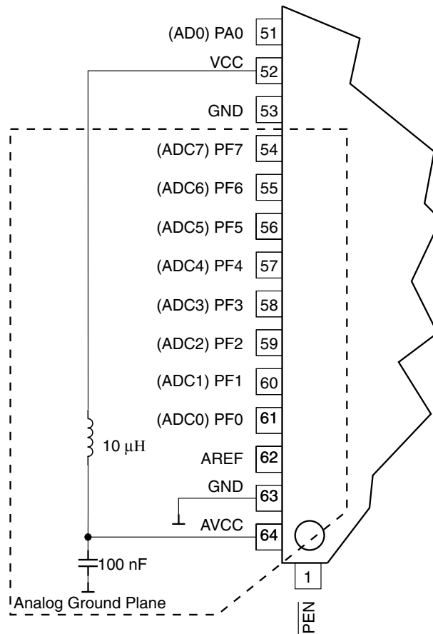
Figure 115. ADC Power Connections
