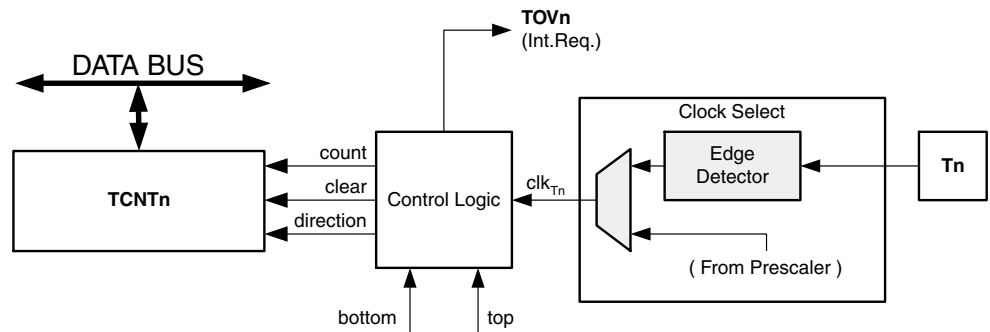
Figure 61. Counter Unit Block Diagram
