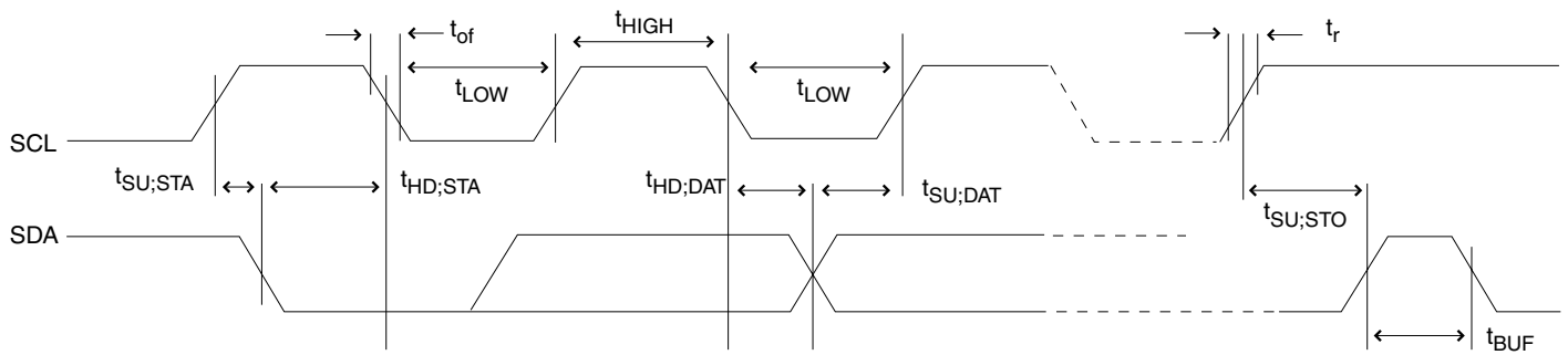
Figure 156. 2-wire Serial Bus Timing
