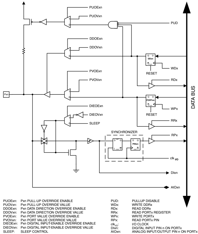
Figure 32. Alternate Port Functions (1)
