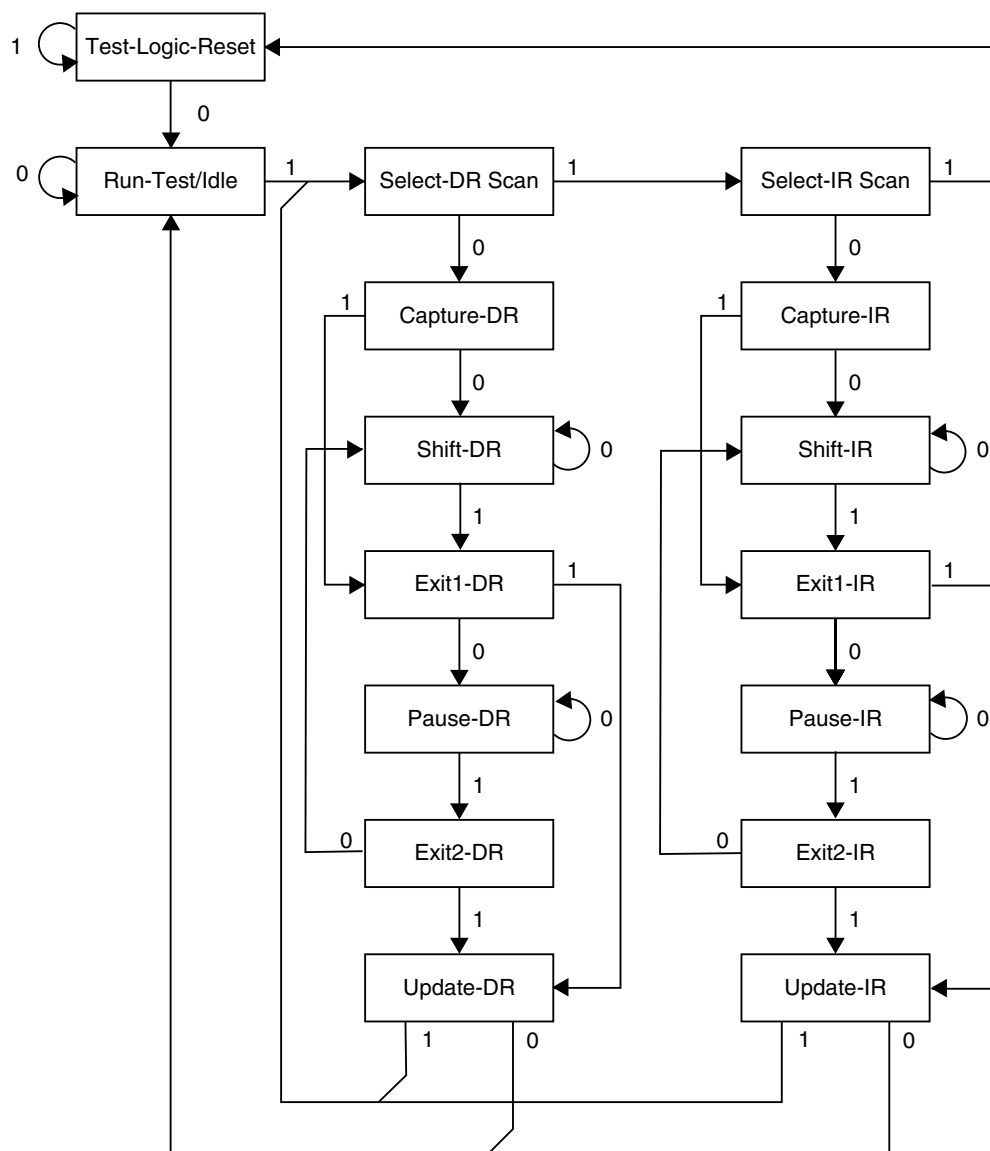
Figure 123. TAP Controller State Diagram
