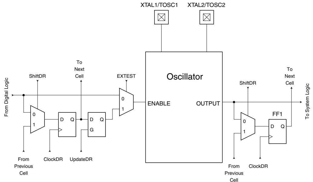
Figure 130. Boundary-scan Cells for Oscillators and Clock Options
