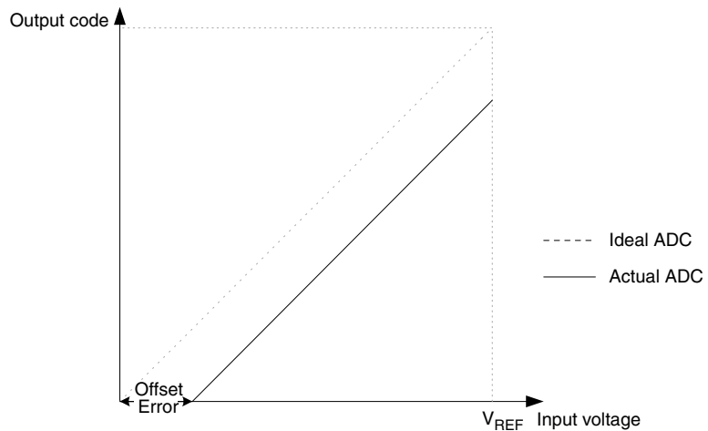
Figure 116. Offset Error
