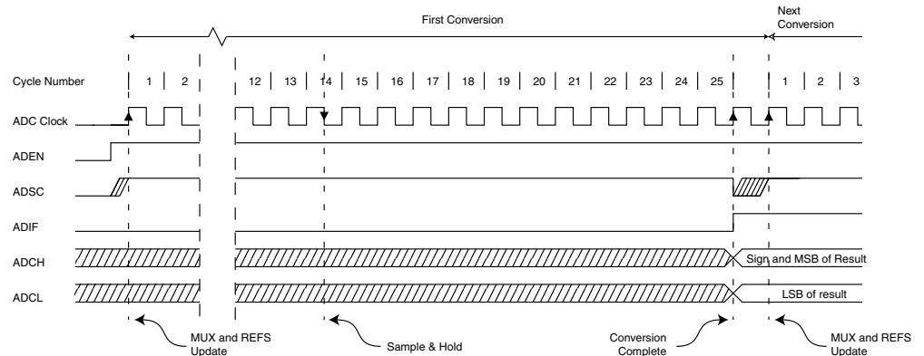
Figure 110. ADC Timing Diagram, First Conversion (Single Conversion Mode)
