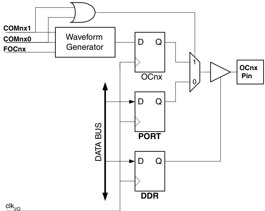
Figure 49. Compare Match Output Unit, Schematic
