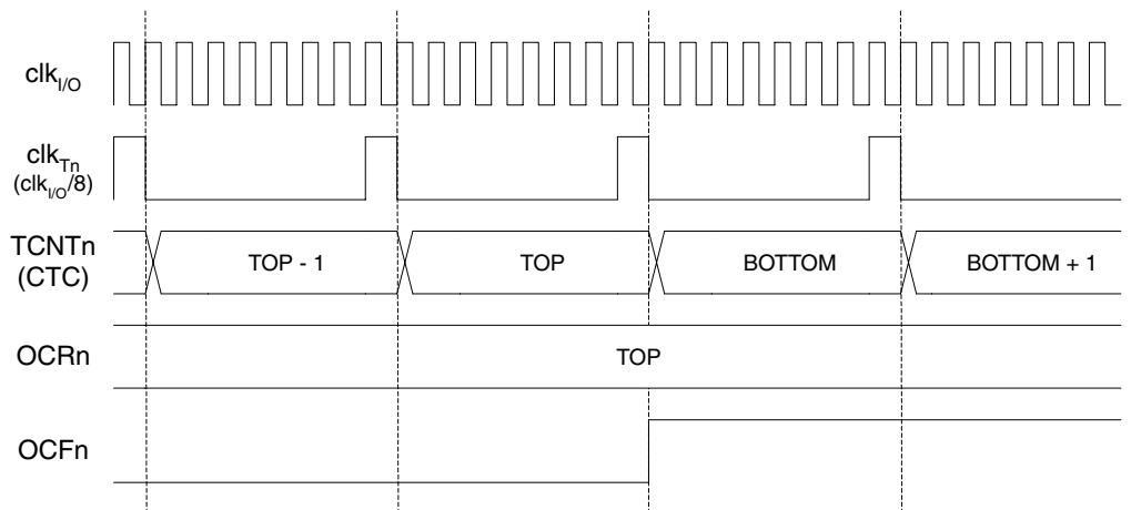
Figure 70. Timer/Counter Timing Diagram, Clear Timer on Compare Match Mode, with Prescaler ( f_{clk\_I/O}/8 )
