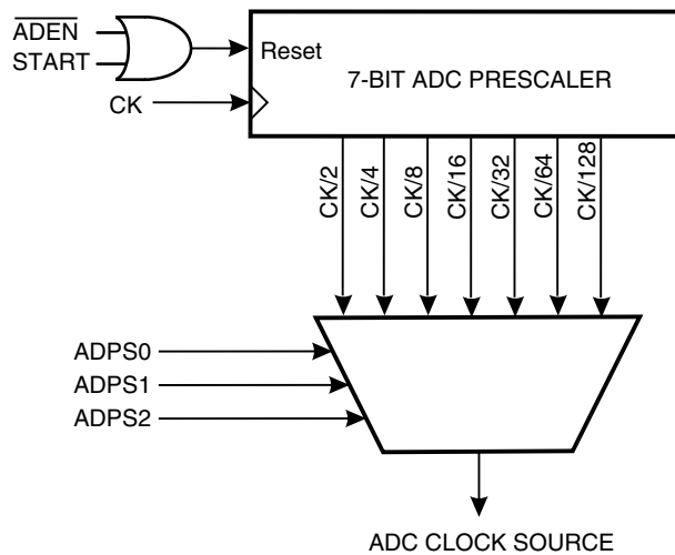
Figure 109. ADC Prescaler
