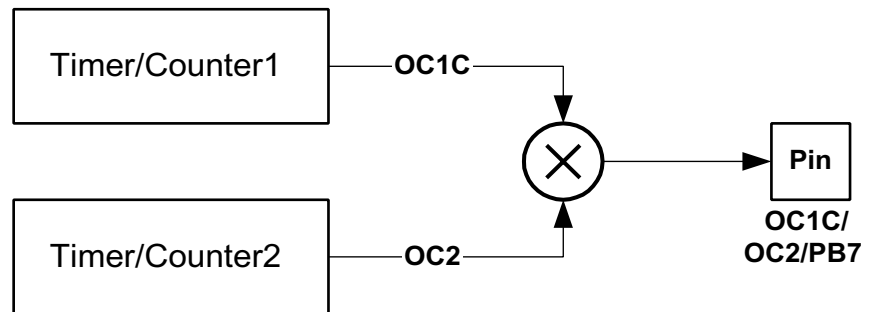
Figure 71. Output Compare Modulator, Block Diagram
