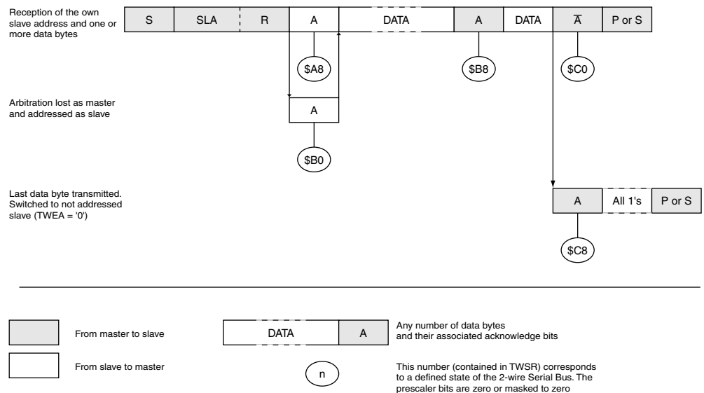
Figure 102. Formats and States in the Slave Transmitter Mode
