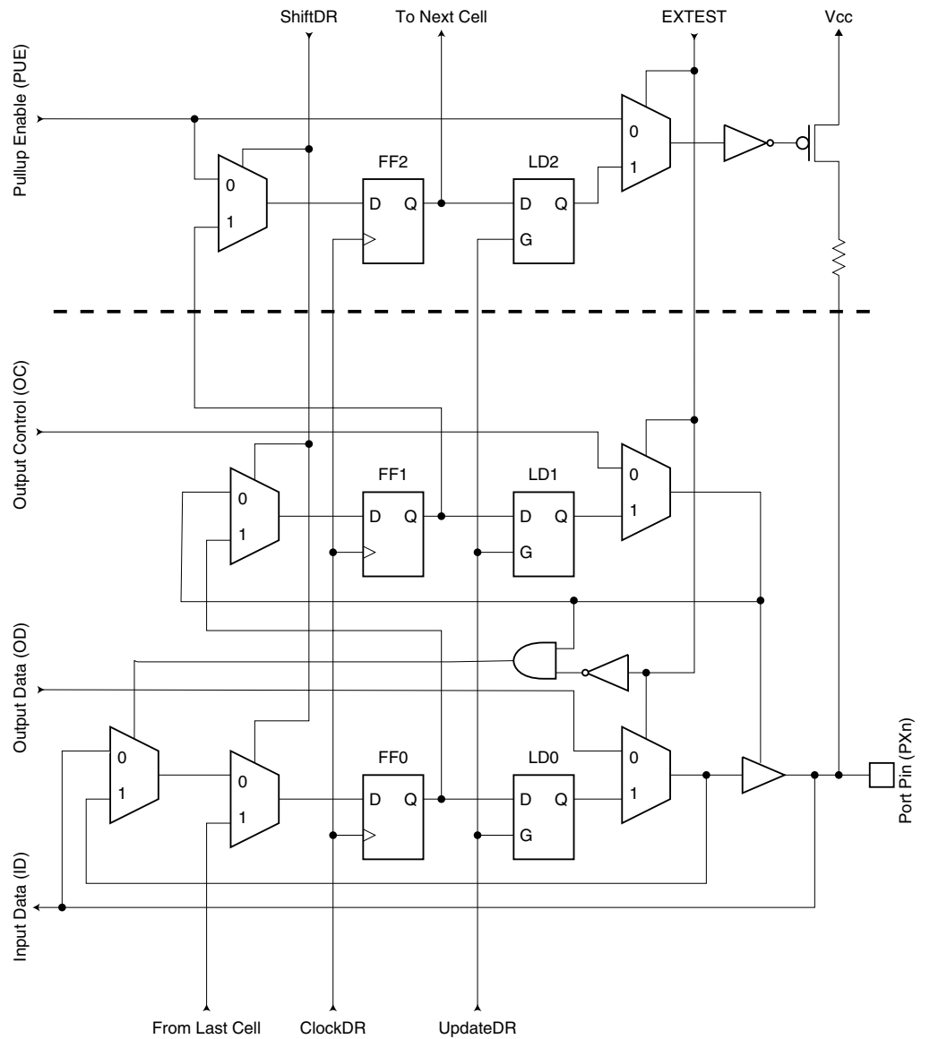
Figure 126. Boundary-scan Cell for Bi-directional Port Pin with Pull-up Function
