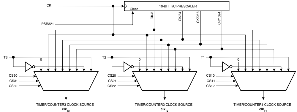
Figure 59. Prescaler for Timer/Counter1, Timer/Counter2, and Timer/Counter3
