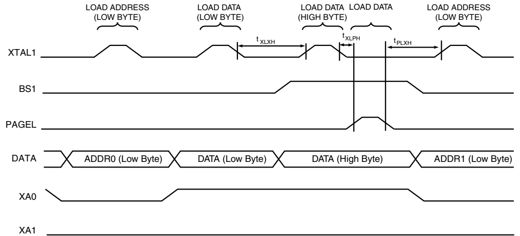
Figure 144. Parallel Programming Timing, Loading Sequence with Timing Requirements (1)
