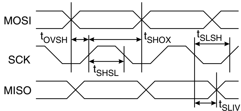
Figure 148. Serial Programming Timing
