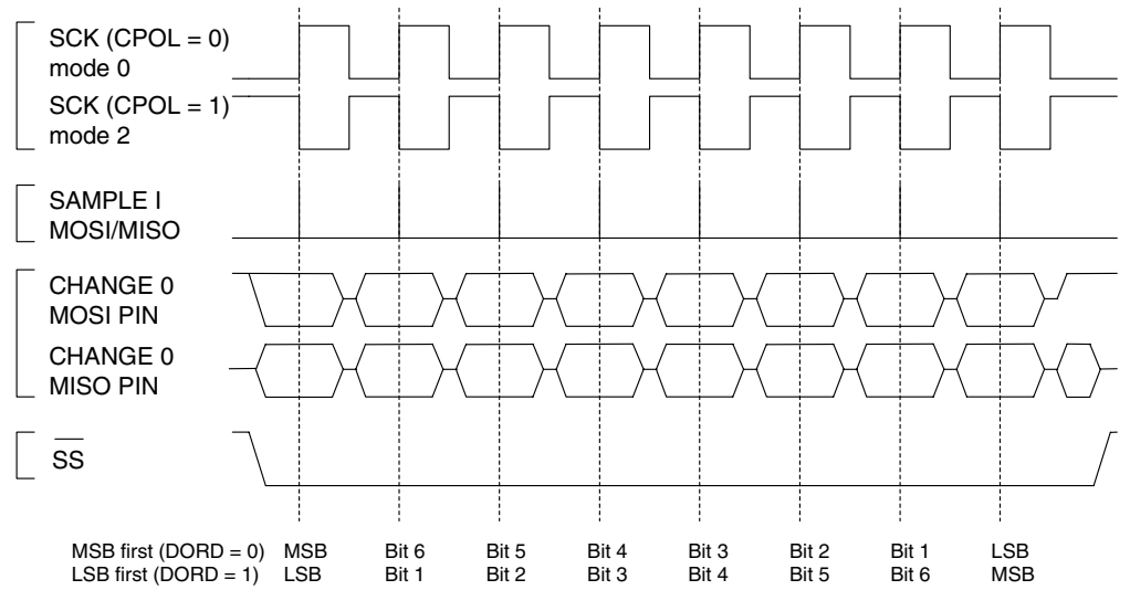
Figure 76. SPI Transfer Format with CPHA = 0
