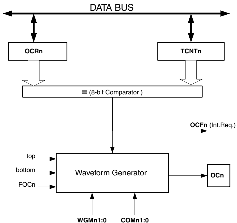
Figure 62. Output Compare Unit, Block Diagram
