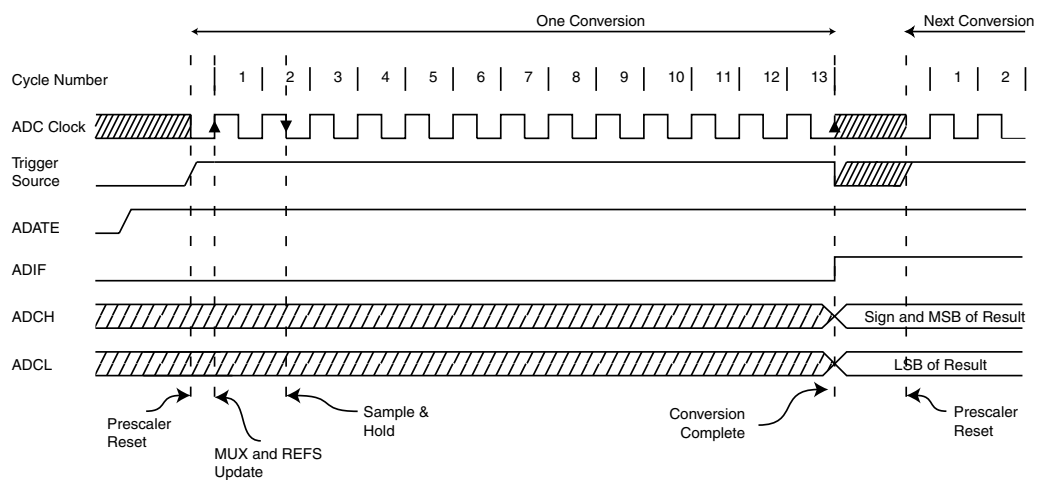
Figure 112. ADC Timing Diagram, Auto Triggered Conversion
