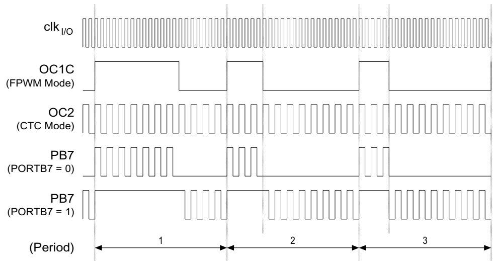
Figure 73. Output Compare Modulator, Timing Diagram
