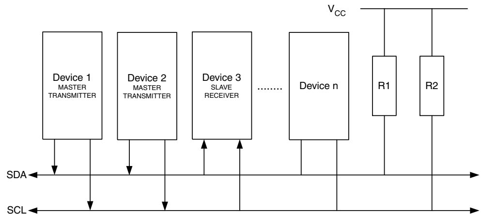
Figure 104. An Arbitration Example
