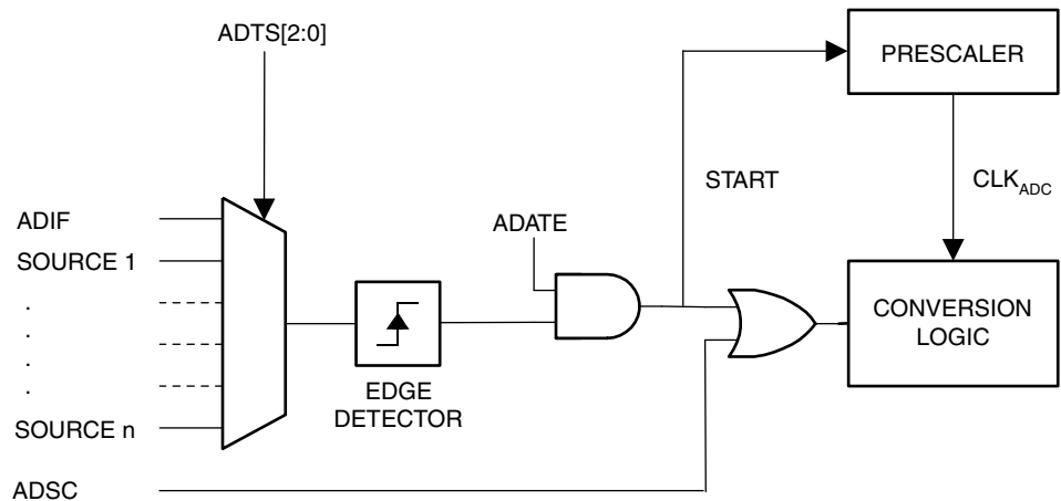
Figure 108. ADC Auto Trigger Logic
