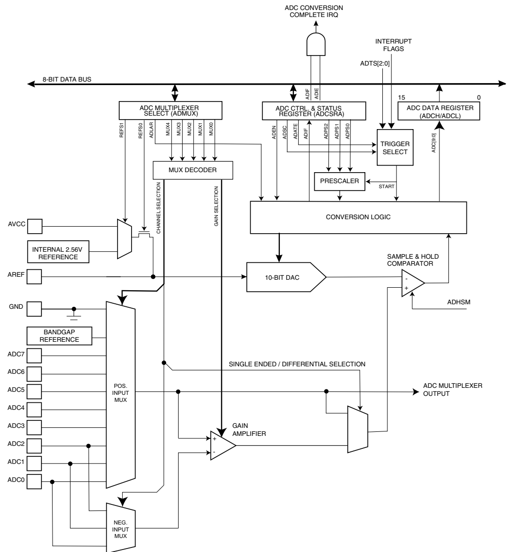
Figure 107. Analog to Digital Converter Block Schematic
