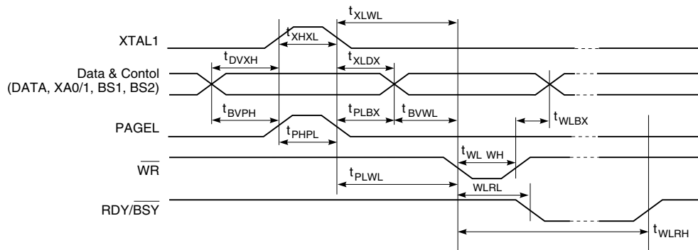
Figure 143. Parallel Programming Timing, Including some General Timing Requirements
