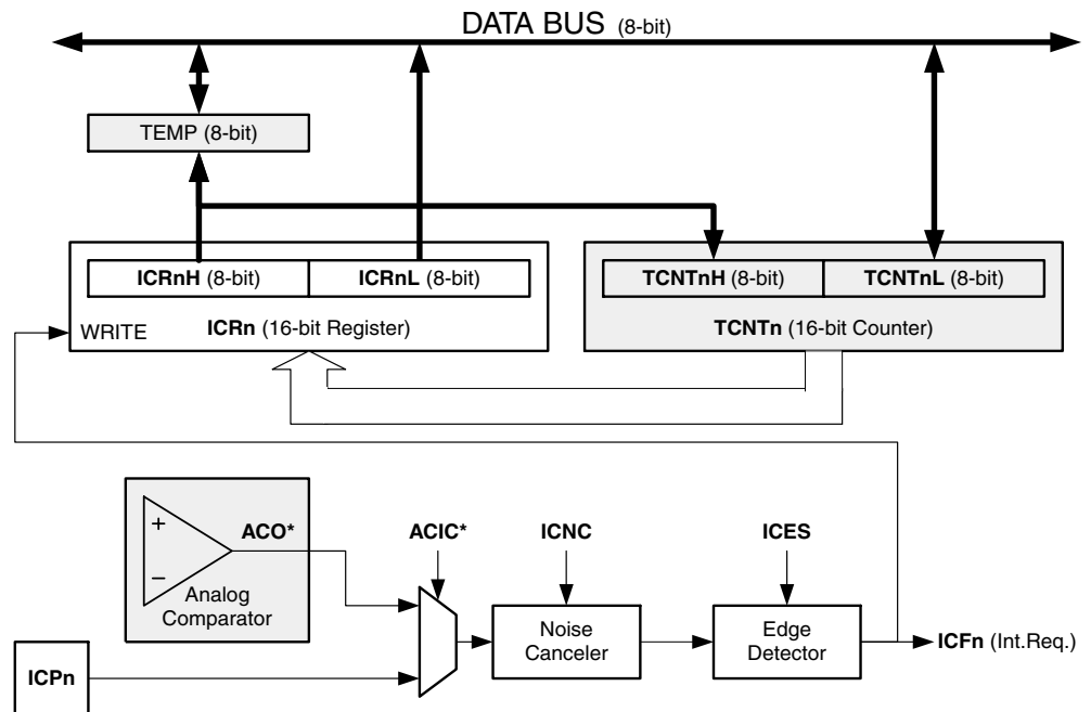
Figure 47. Input Capture Unit Block Diagram (1)
