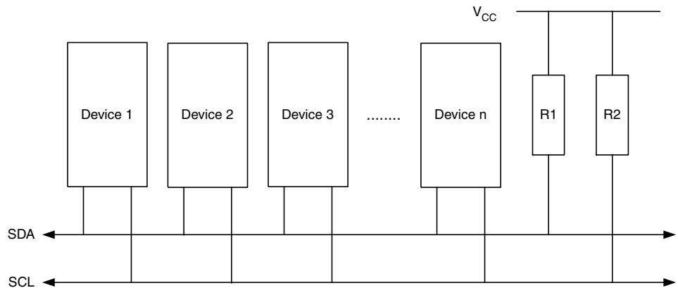
Figure 85. TWI Bus Interconnection
