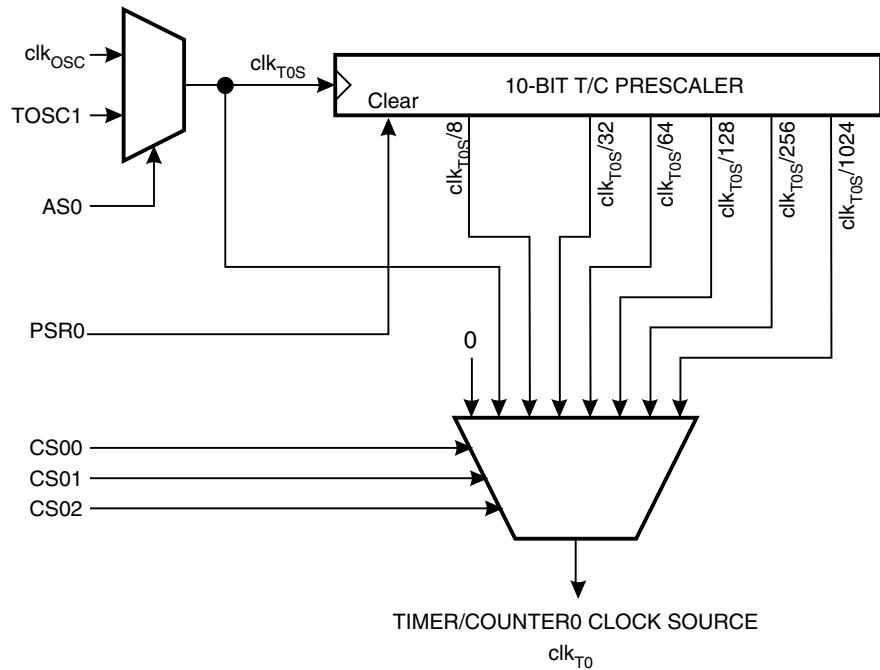
Timer/Counter Prescaler Figure 44. Prescaler for Timer/Counter0
