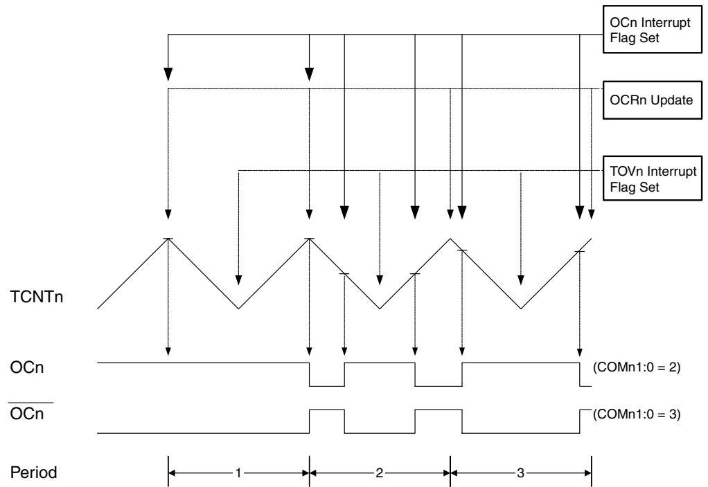
Figure 66. Phase Correct PWM Mode, Timing Diagram
