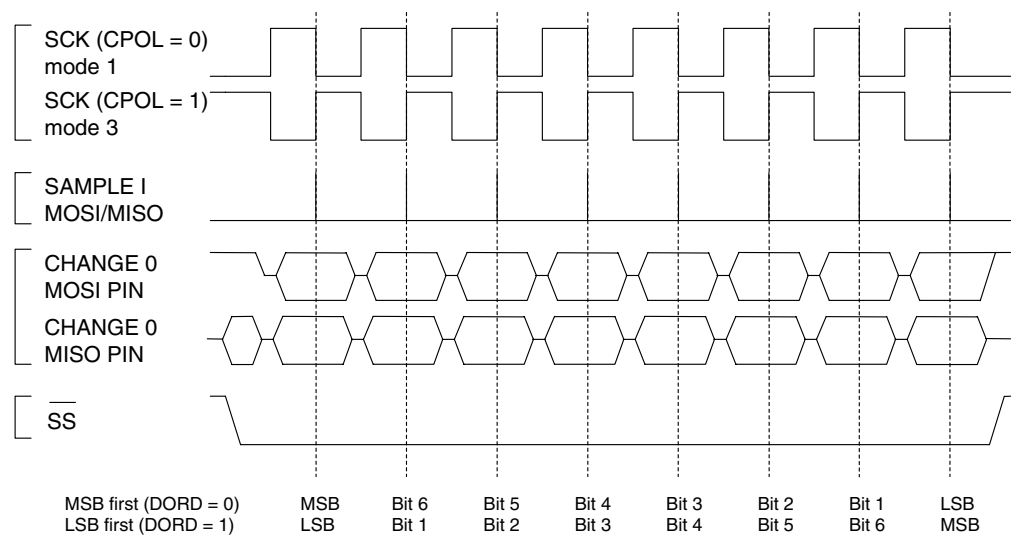
Figure 77. SPI Transfer Format with CPHA = 1
