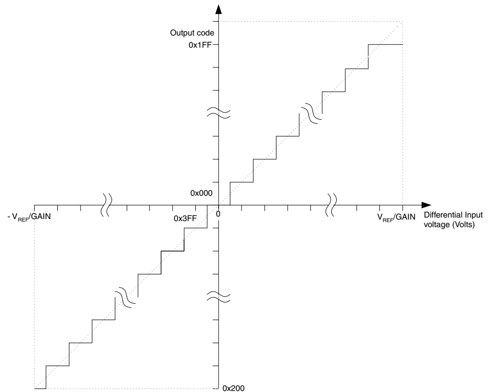
Figure 120. Differential Measurement Range
