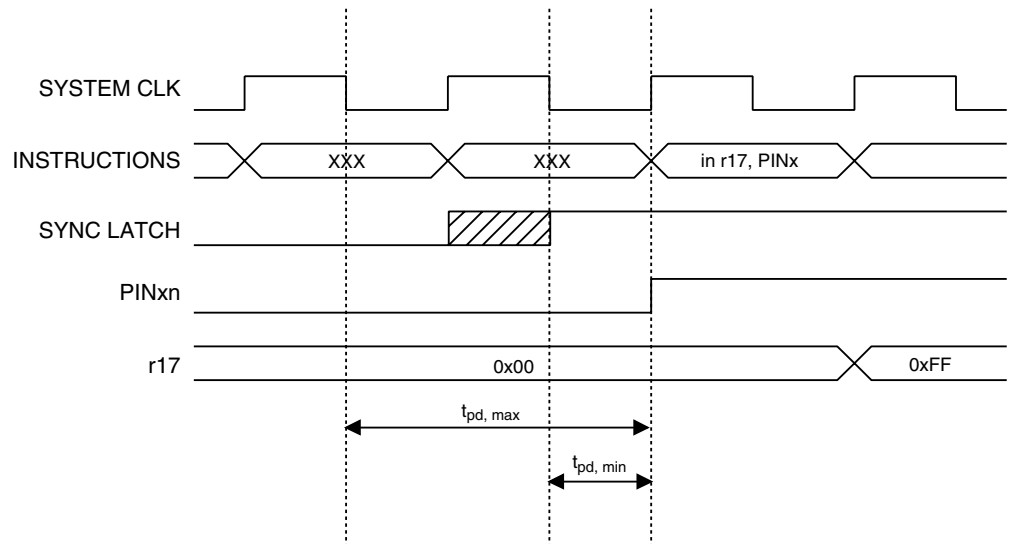
Figure 30. Synchronization when Reading an Externally Applied Pin Value
