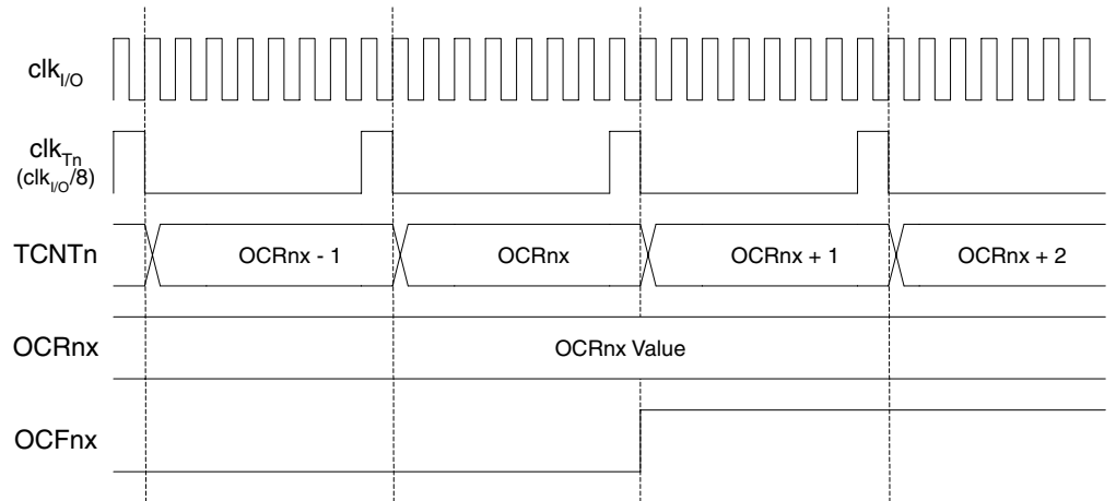
Figure 55. Timer/Counter Timing Diagram, Setting of OCFnx, with Prescaler ( f_{clk\_I/O}/8 )
