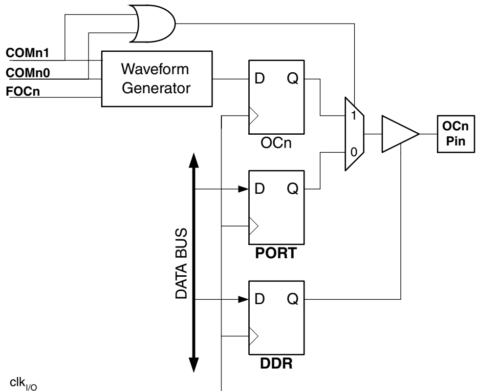
Figure 36. Compare Match Output Unit, Schematic
