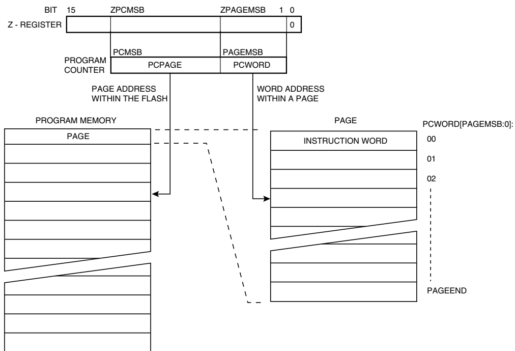
Figure 137. Addressing the Flash during SPM (1)
