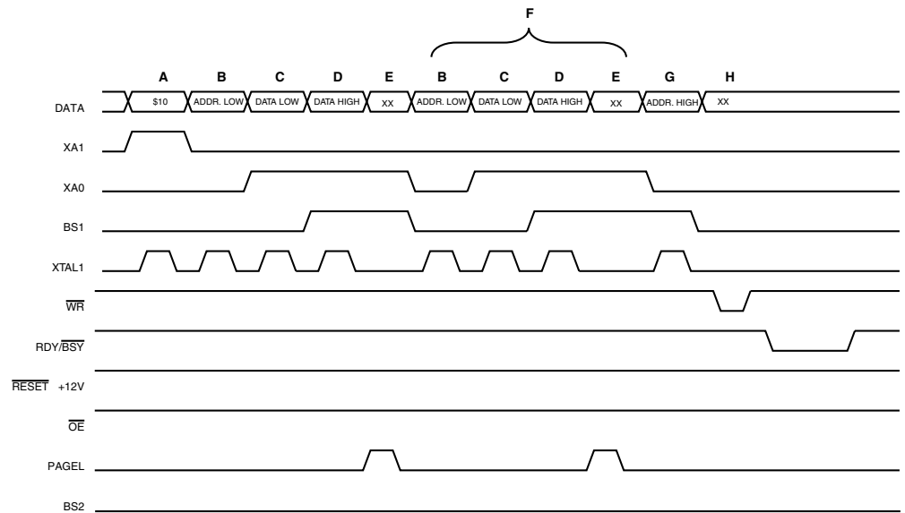
Figure 140. Programming the Flash Waveforms
