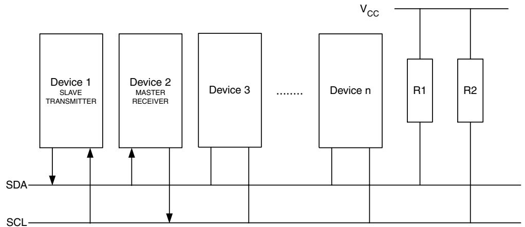
Figure 101. Data Transfer in Slave Transmitter Mode
