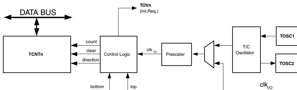
Figure 34. Counter Unit Block Diagram
