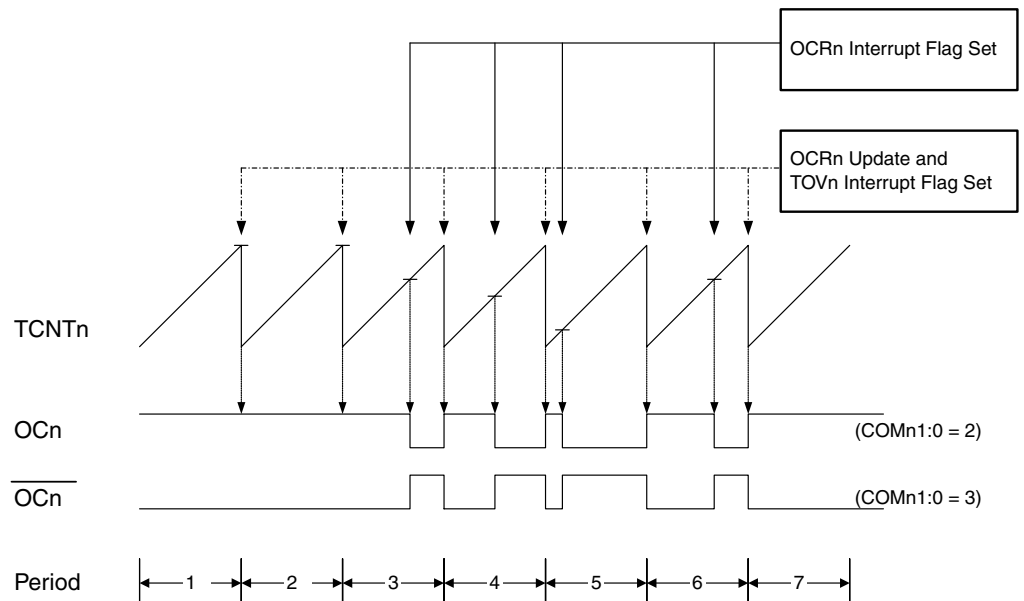
Figure 38. Fast PWM Mode, Timing Diagram
