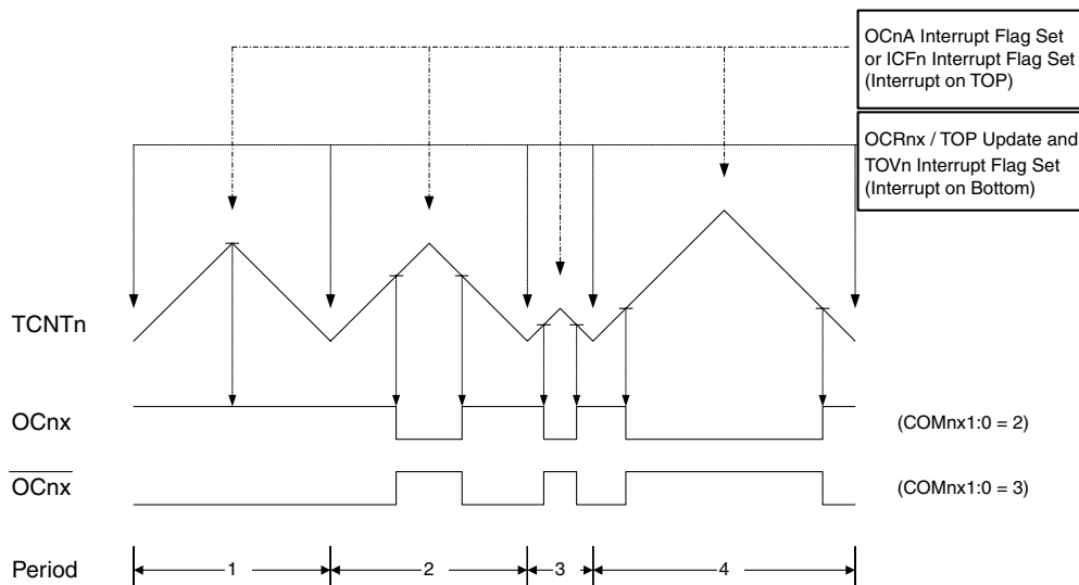
Figure 53. Phase and Frequency Correct PWM Mode, Timing Diagram
