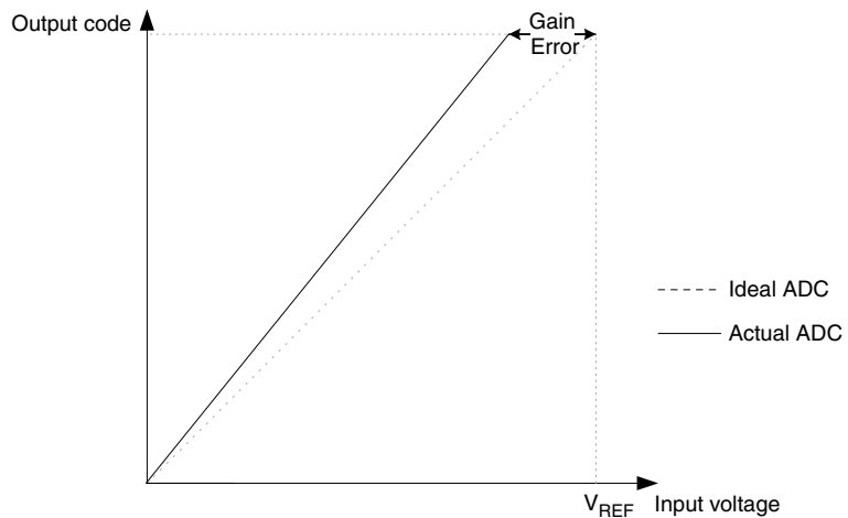
Figure 117. Gain Error
