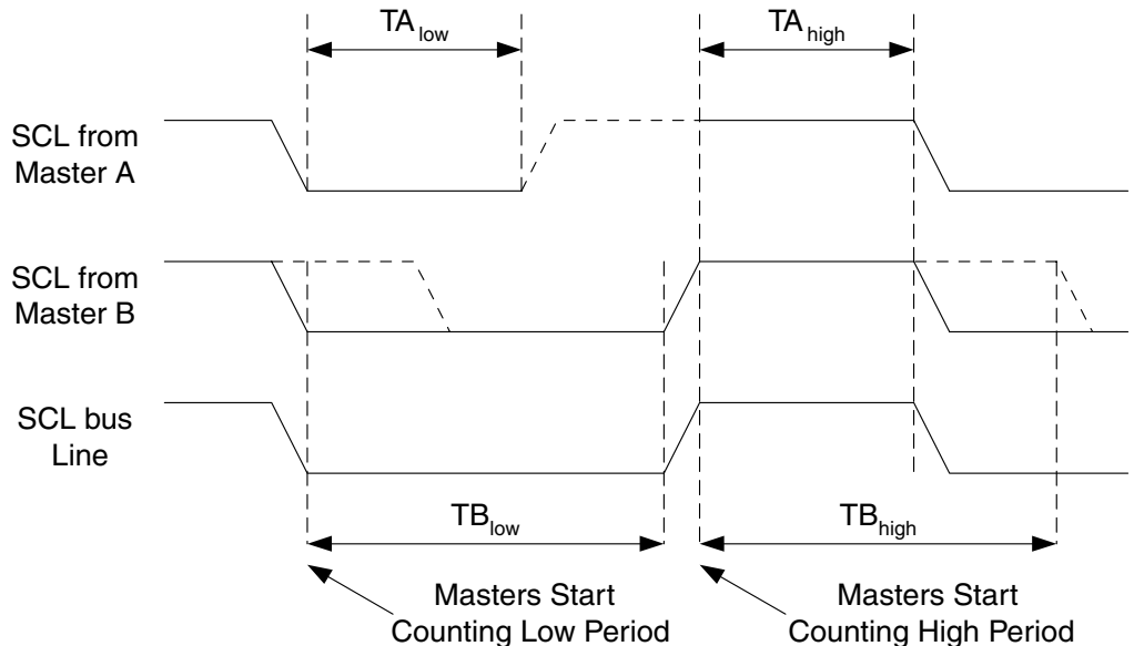
Figure 91. SCL Synchronization between Multiple Masters
