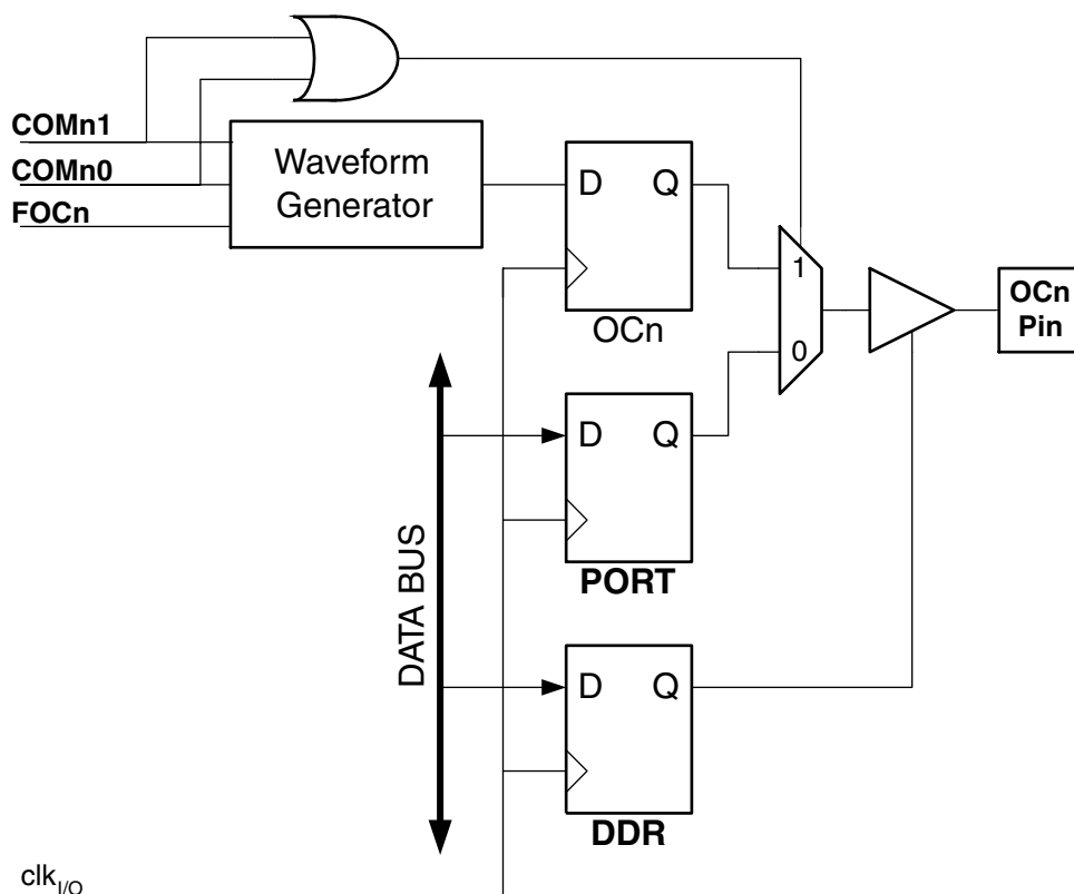
Figure 63. Compare Match Output Unit, Schematic
