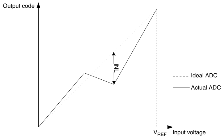
Figure 118. Integral Non-linearity (INL)
