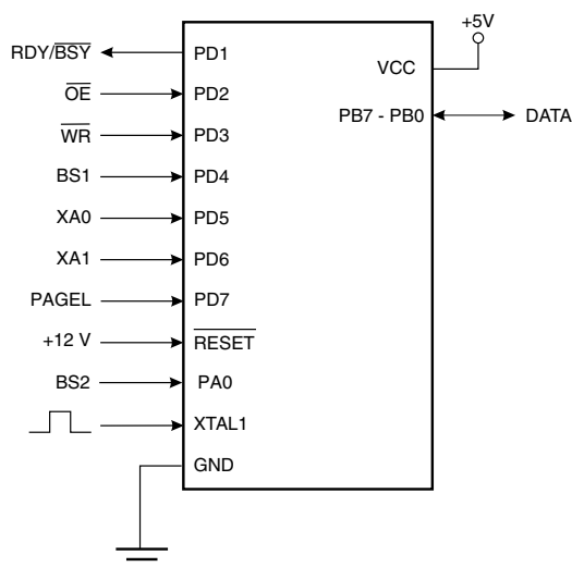
Figure 138. Parallel Programming
