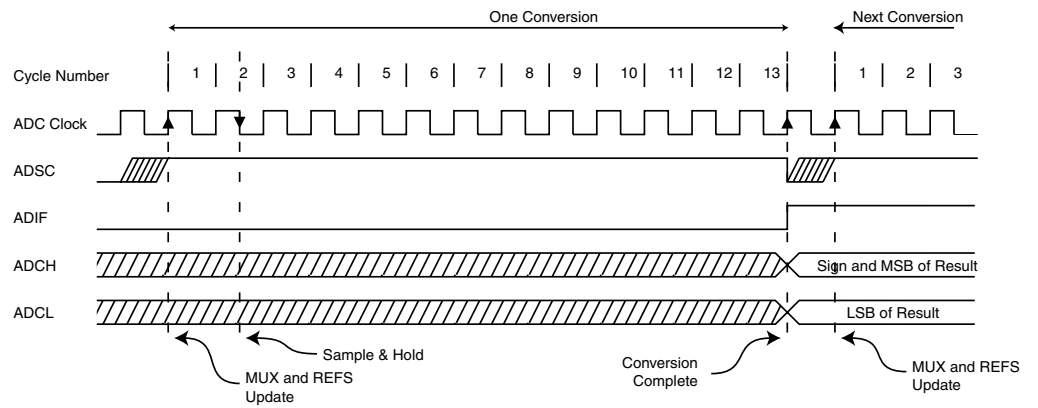
Figure 111. ADC Timing Diagram, Single Conversion
