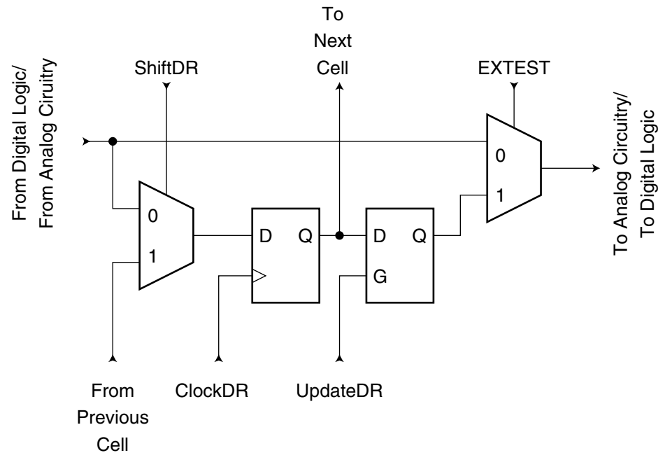
Figure 132. General Boundary-scan Cell used for Signals for Comparator and ADC
