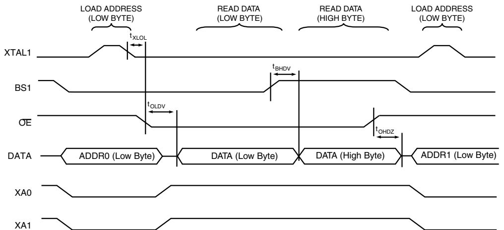
Figure 145. Parallel Programming Timing, Reading Sequence (Within the Same Page) with Timing Requirements (1)
