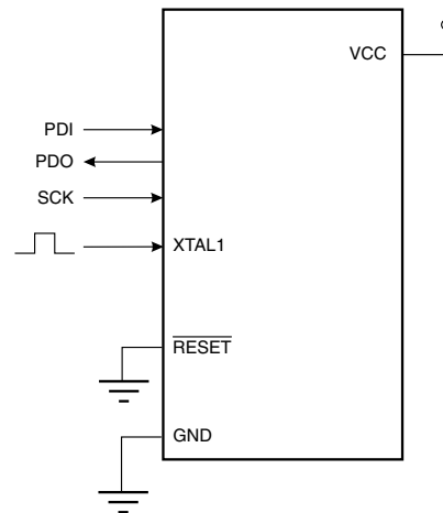
Figure 146. Serial Programming and Verify (1)
