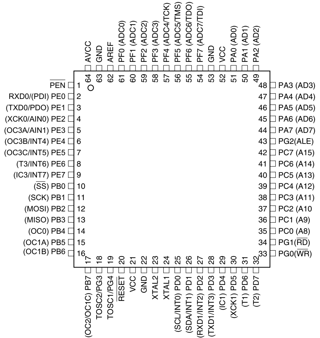
Figure 1. Pinout ATmega64
