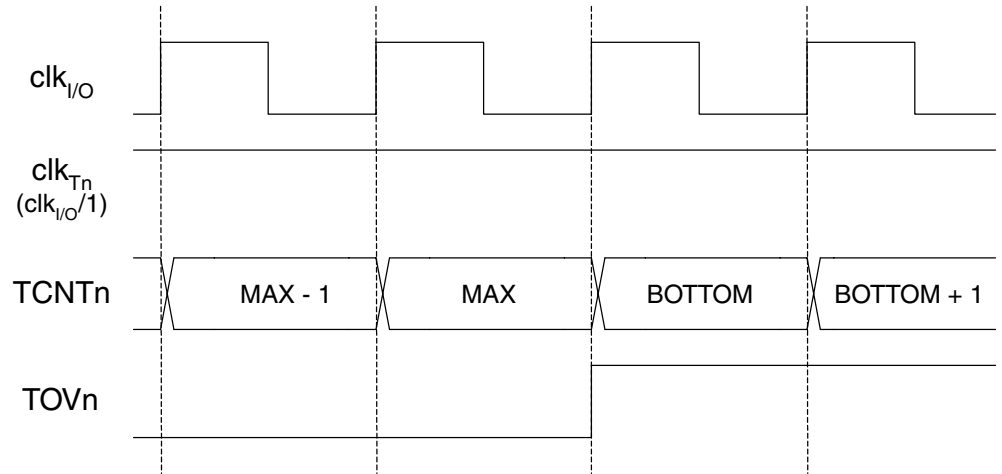
Figure 67. Timer/Counter Timing Diagram, no Prescaling
