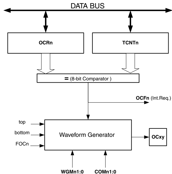
Figure 35. Output Compare Unit, Block Diagram
