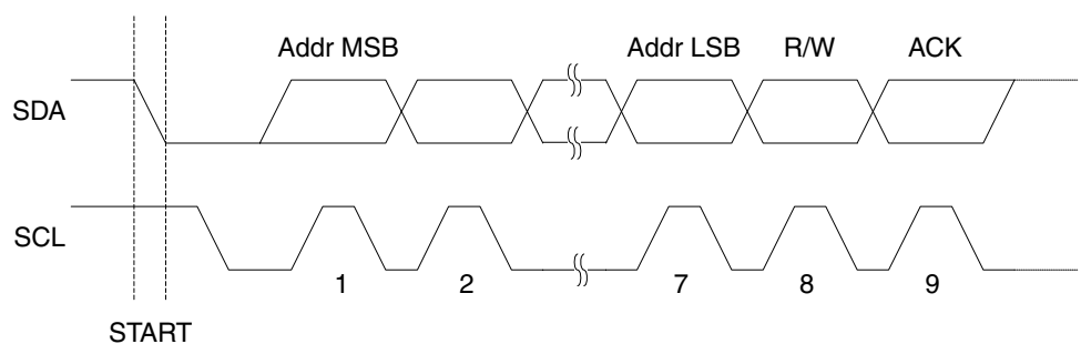
Figure 88. Address Packet Format
