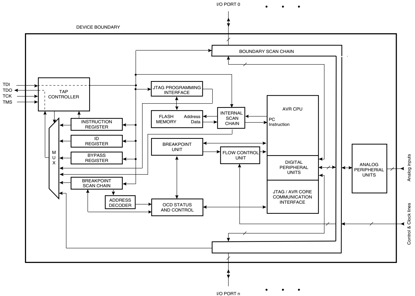
Figure 122. Block Diagram
