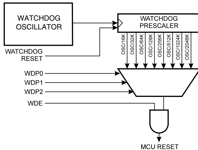
Figure 27. Watchdog Timer
