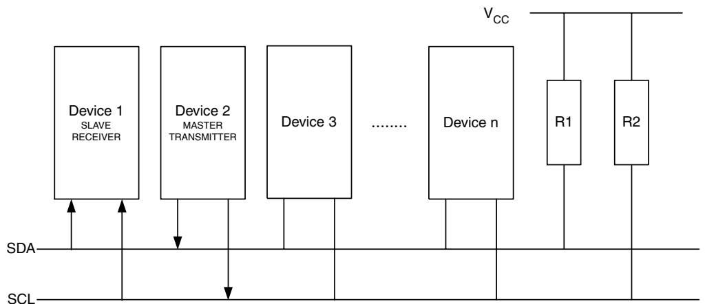
Figure 99. Data Transfer in Slave Receiver Mode
