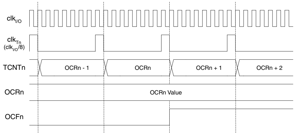
Figure 69. Timer/Counter Timing Diagram, Setting of OCF2, with Prescaler ( f_{clk\_I/O}/8 )
