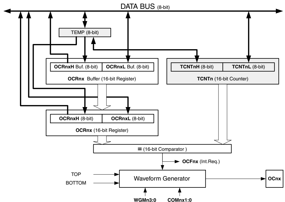
Figure 48. Output Compare Unit, Block Diagram
