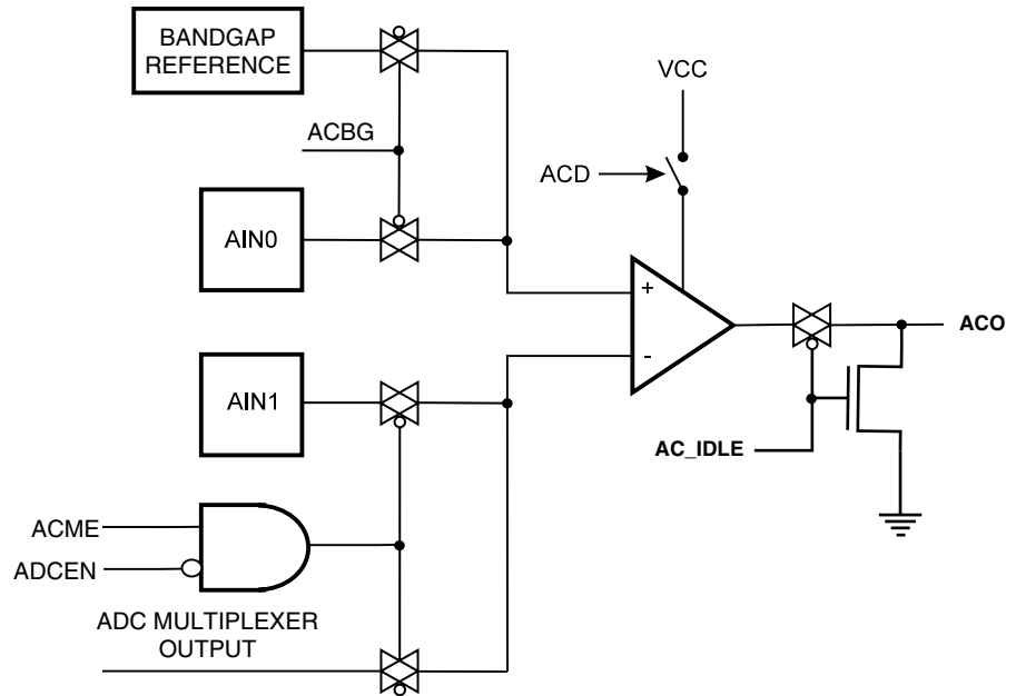
Figure 131. Analog Comparator
