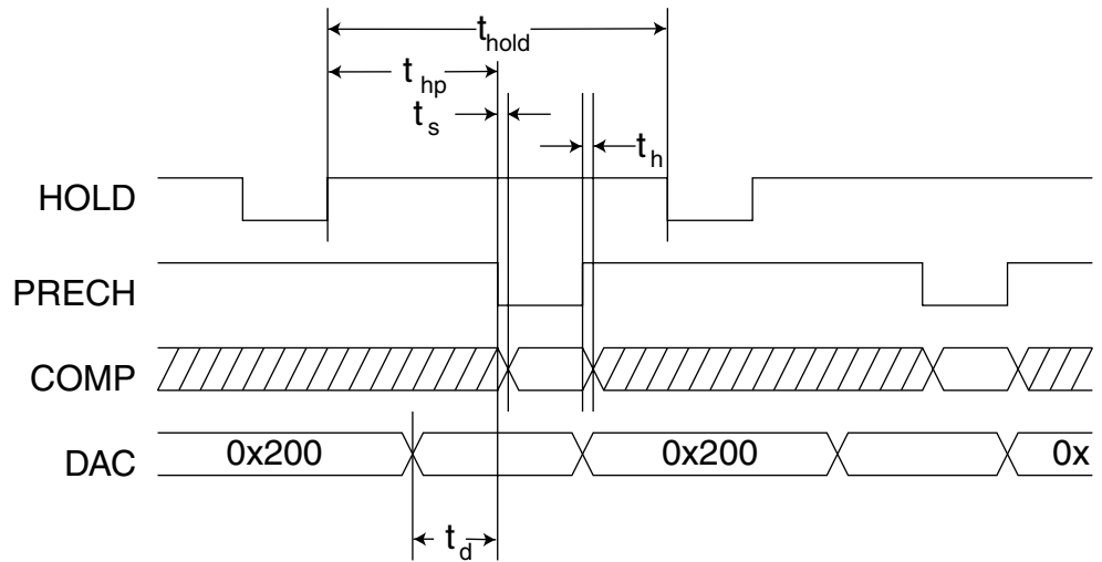
Figure 134. ADC Timing Diagram and Timing Constraints
