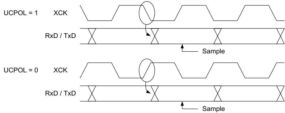
Figure 80. Synchronous Mode XCK Timing
