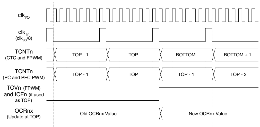
Figure 57. Timer/Counter Timing Diagram, with Prescaler ( f_{clk\_I/O}/8 )
