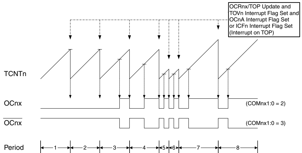
Figure 51. Fast PWM Mode, Timing Diagram
