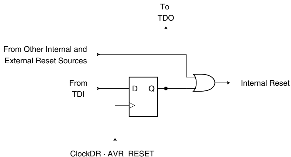
Figure 125. Reset Register
