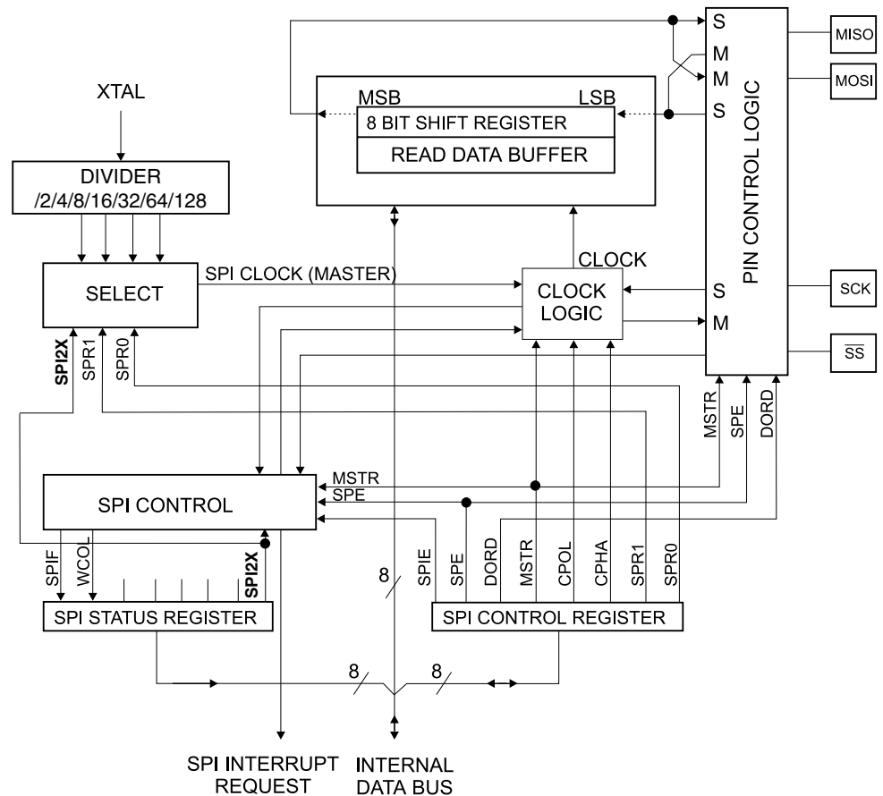
Figure 74. SPI Block Diagram (1)
