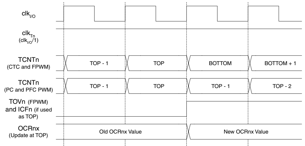
Figure 56. Timer/Counter Timing Diagram, no Prescaling
