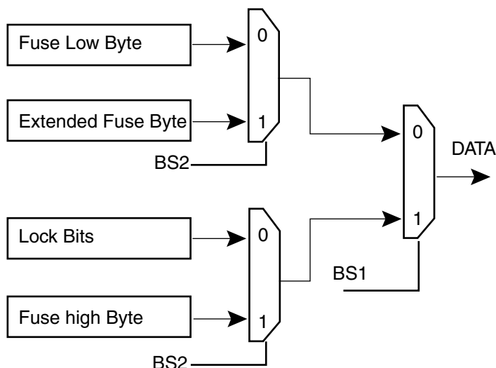
Figure 142. Mapping Between BS1, BS2 and the Fuse and Lock Bits during Read
