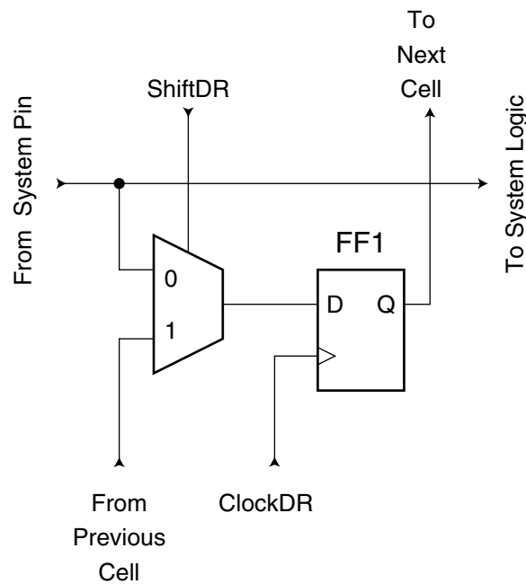
Figure 129. Observe-only Cell
