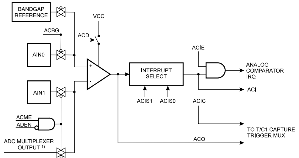
Figure 106. Analog Comparator Block Diagram (1)(2)
