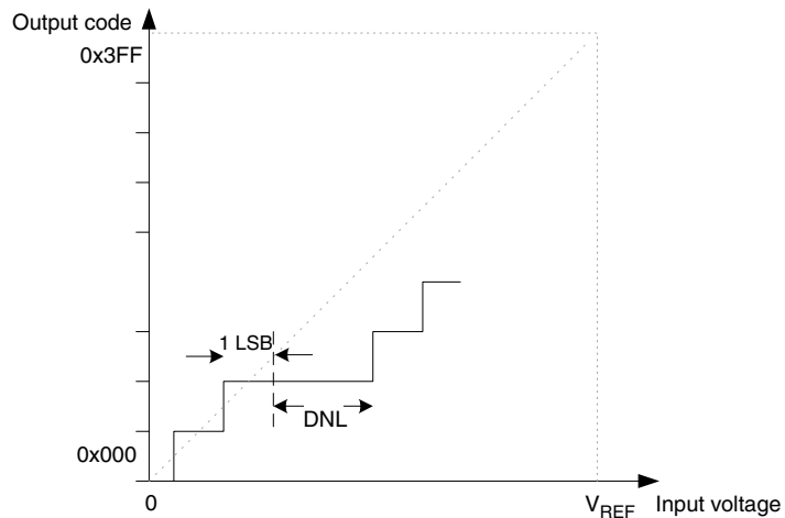
Figure 119. Differential Non-linearity (DNL)
