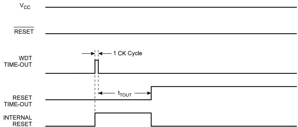
Figure 26. Watchdog Reset During Operation
