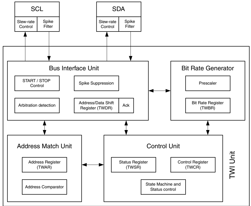
Figure 93. Overview of the TWI Module
