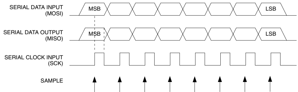
Figure 147. .Serial Programming Waveforms
