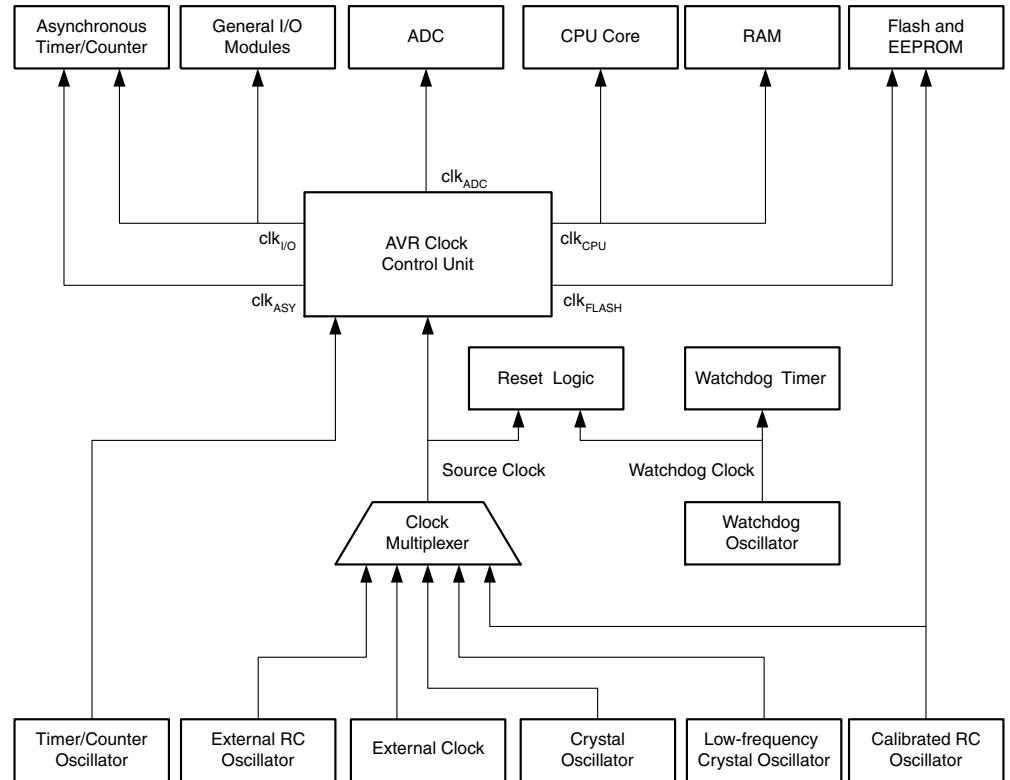
Figure 17. Clock Distribution
