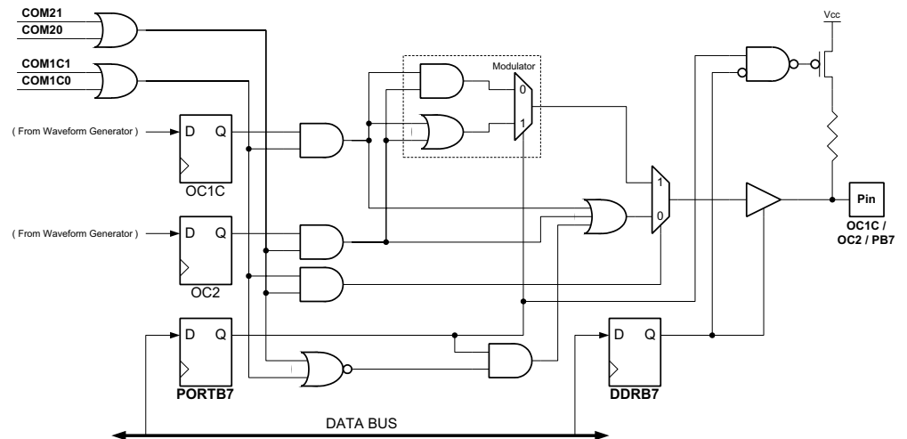
Figure 72. Output Compare Modulator, Schematic
