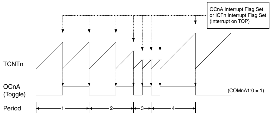
Figure 50. CTC Mode, Timing Diagram
