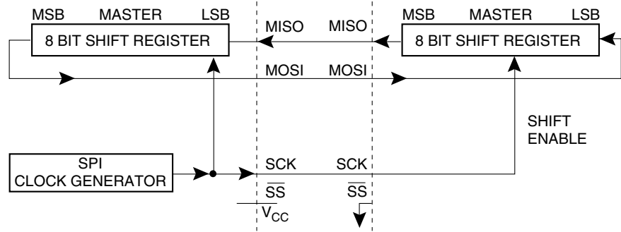
Figure 75. SPI Master-Slave Interconnection
