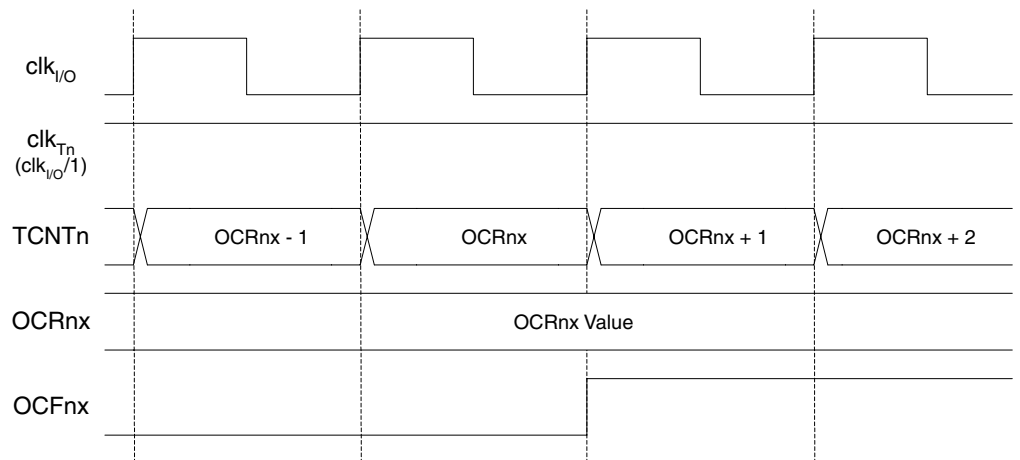
Figure 54. Timer/Counter Timing Diagram, Setting of OCFnx, no Prescaling
