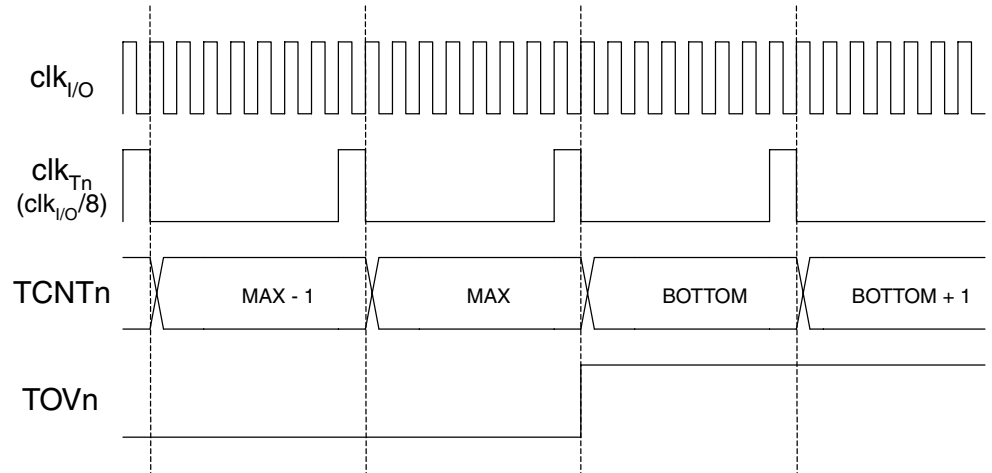
Figure 68. Timer/Counter Timing Diagram, with Prescaler ( f_{clk_{I/O}}/8 )
