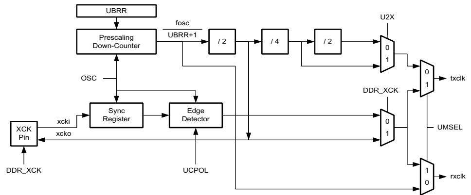
Figure 79. Clock Generation Logic, Block Diagram
