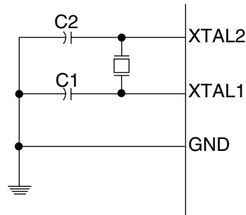
Figure 18. Crystal Oscillator Connections
