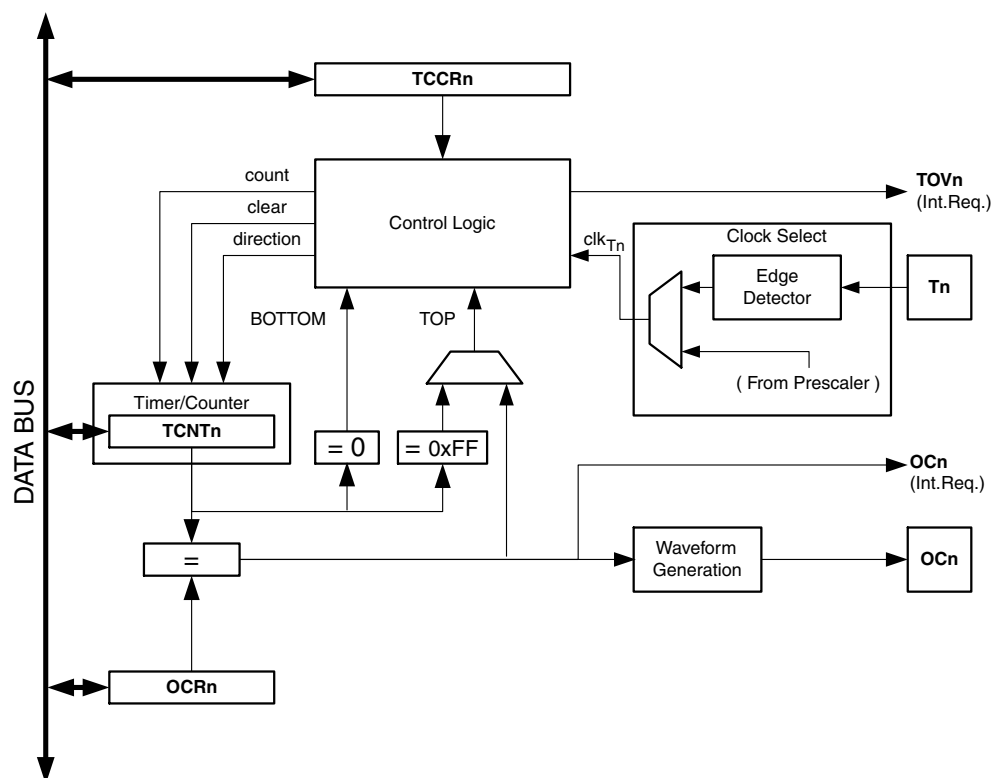
Figure 60. 8-bit Timer/Counter Block Diagram
