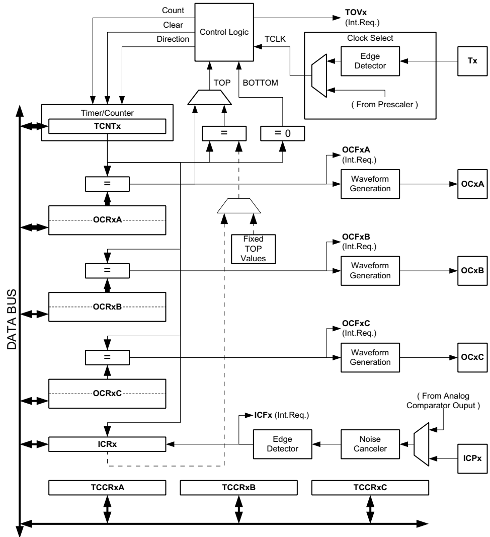
Figure 45. 16-bit Timer/Counter Block Diagram (1)
