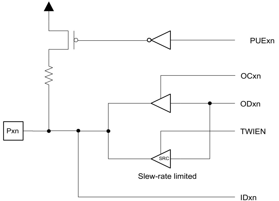
Figure 128. Additional Scan Signal for the Two-wire Interface
