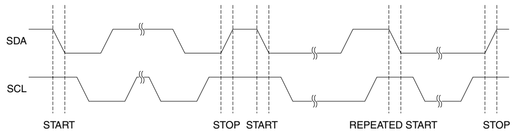
Figure 87. START, REPEATED START and STOP Conditions
