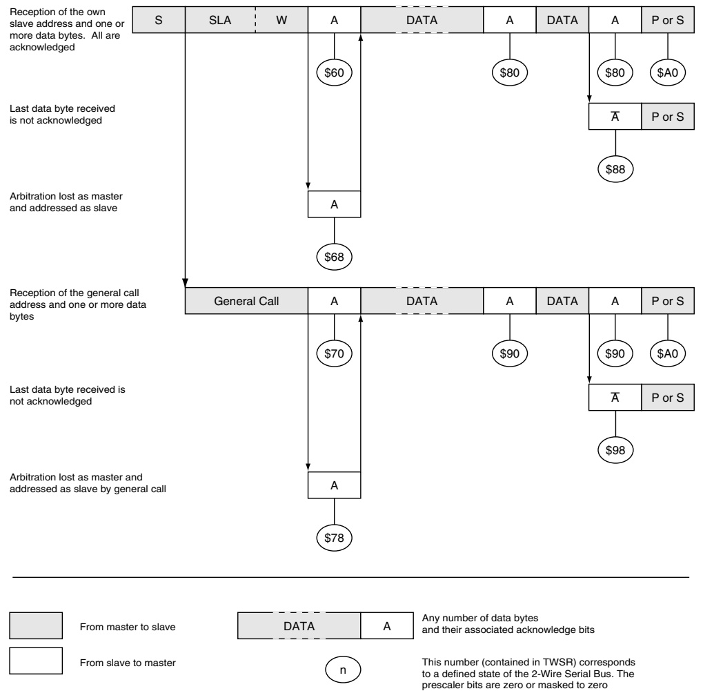
Figure 100. Formats and States in the Slave Receiver Mode
