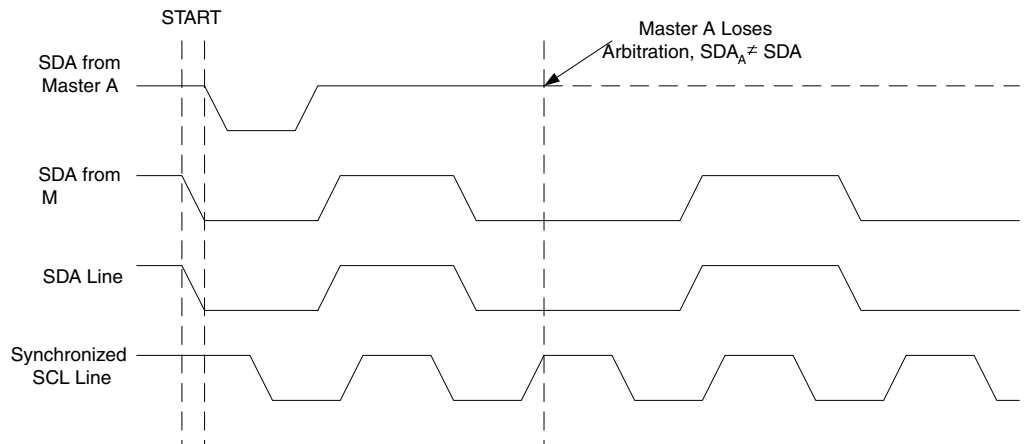
Figure 92. Arbitration between two Masters
