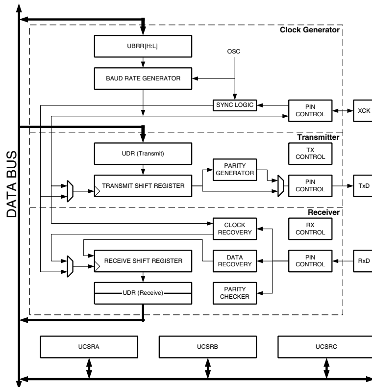
Figure 78. USART Block Diagram (1)
